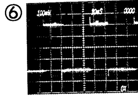
IC201 Pin ②⑨ Record Control (-) (100mV/10msec)
