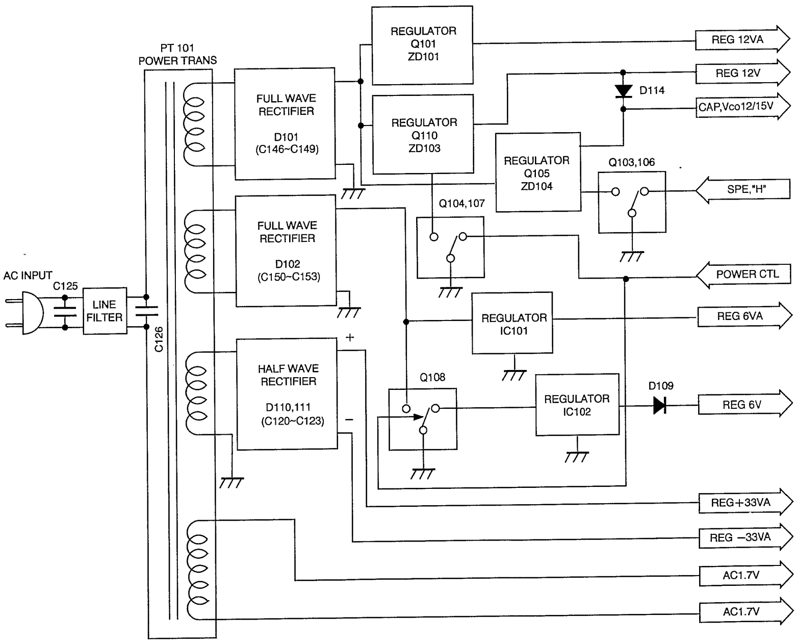
BLOCK DIAGRAMS 1. Power Block Diagram
