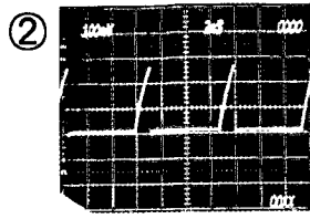
IC201 Pin ⑥ PG Mono-Multi (100mV/2msec)
