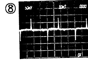
IC201 Pin ③⑤ Playback Control Pulse (50mV/10msec)
