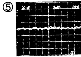
IC201 Pin ②⑦ Capstan Control (20mV/2msec)
