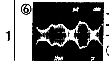
IC703 Pin 5 (20mV/1msec)
