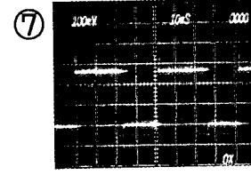
IC201 Pin ③⑩ Record Control (+) (100mV/10msec)
