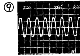
IC201 Pin ③⑦ Capstan Frequency Generator Input (100mV/500 \mu sec)
