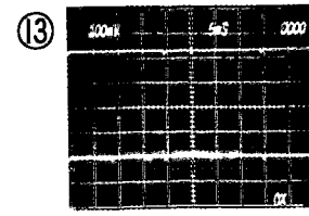
IC201 Pin ⑤⑩ C-SYNC Input terminal (100mV/5msec)
