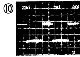
IC201 Pin ③⑨ Control Clock (200mV/10msec)
