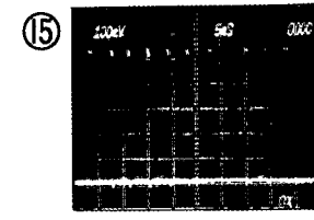
IC201 PIN ⑤④ Servo Clock Input terminal (100mV/5msec)
